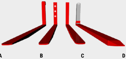
A - PIN-TYPE FORKS B - BOLTED FORKS C - WELDED FORKS D - TELESCOPIC FORKS
